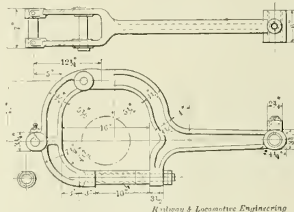
ECCENTRIC ROD EXTENSION—L. & N. RY.
